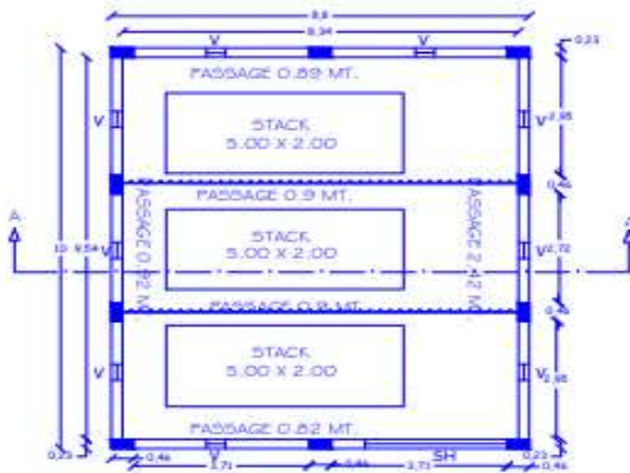
GODOWN PLAN SCALE 1:100
